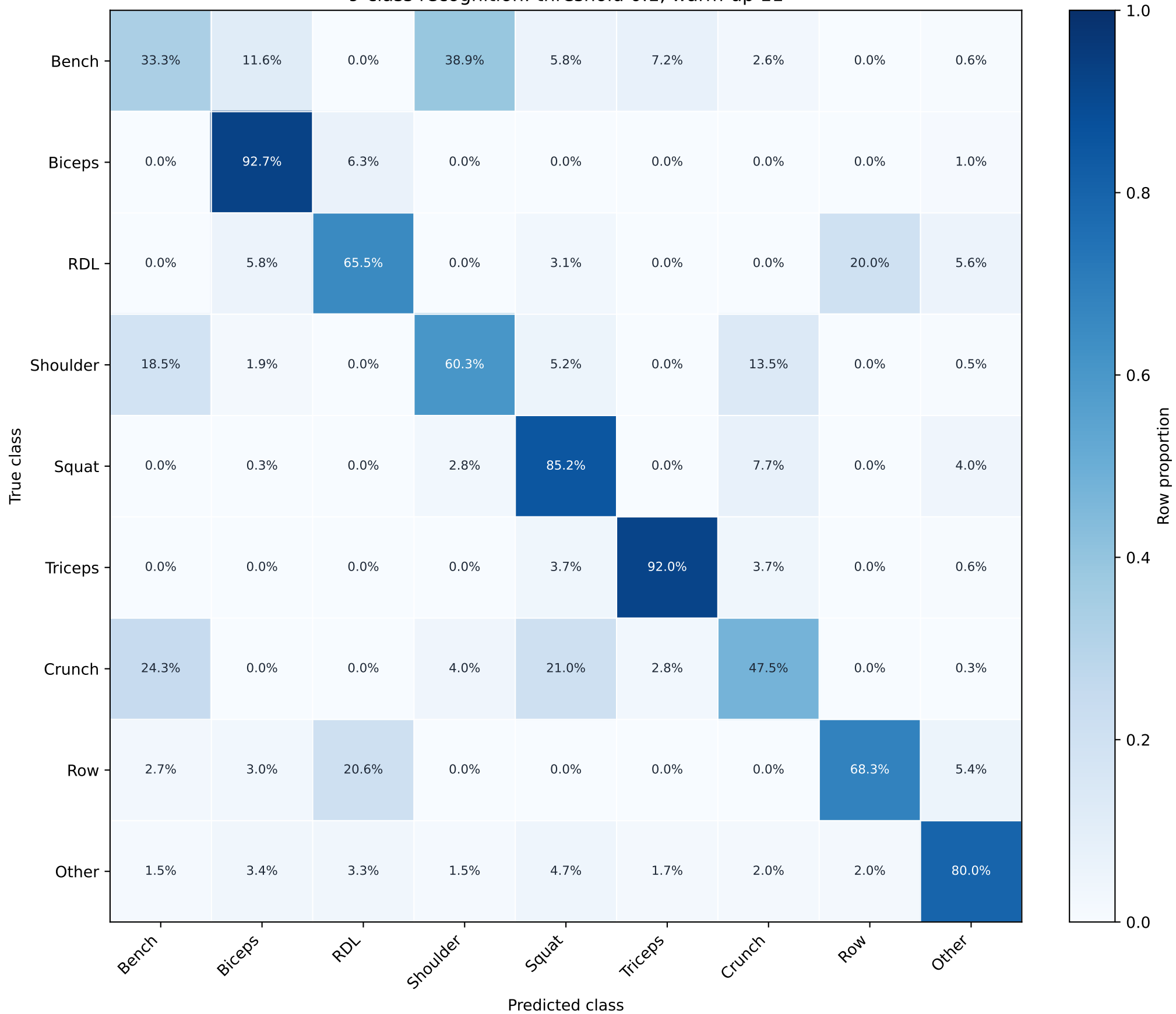
9-class recognition: threshold 0.1, warm-up 11
