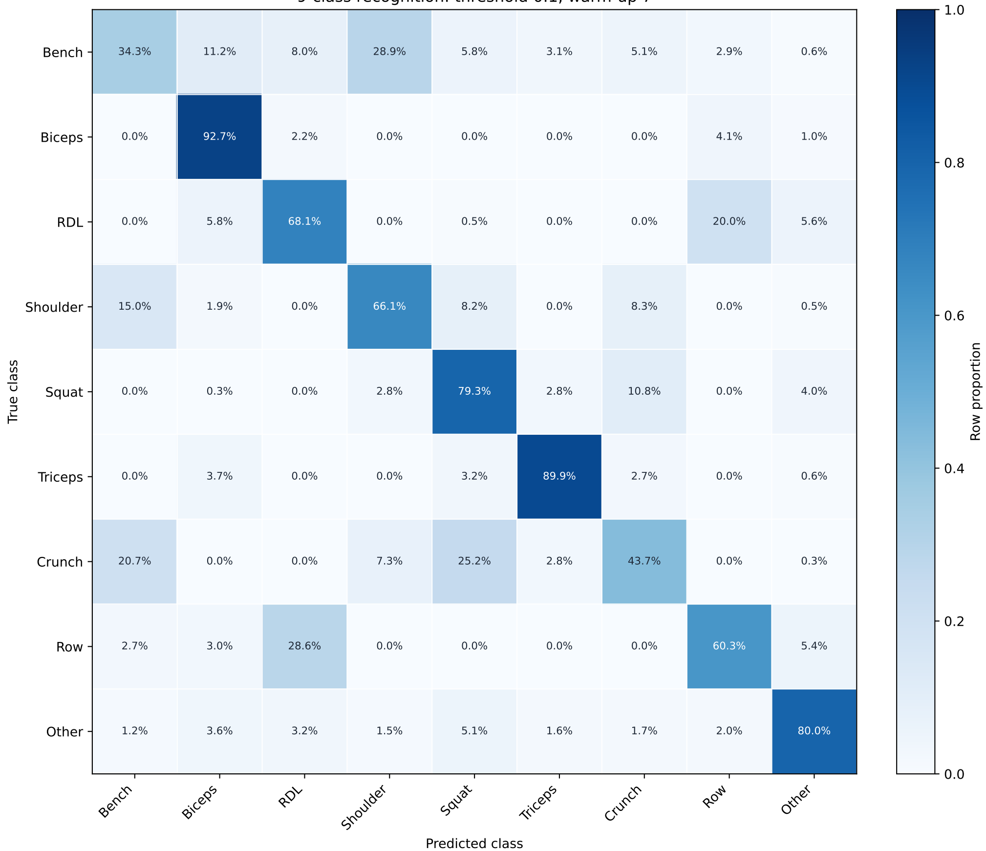
9-class recognition: threshold 0.1, warm-up 7
