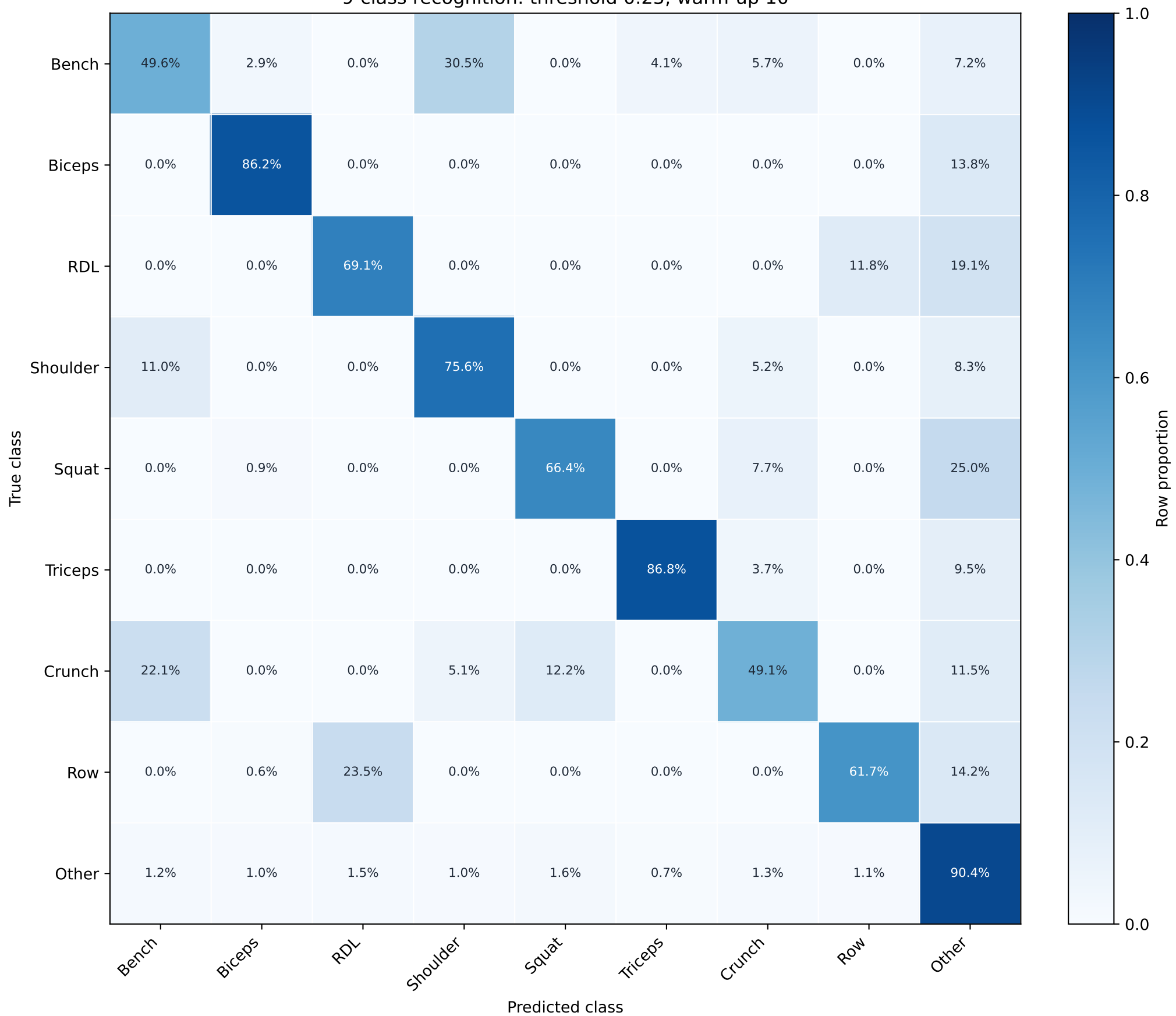
9-class recognition: threshold 0.25, warm-up 10
