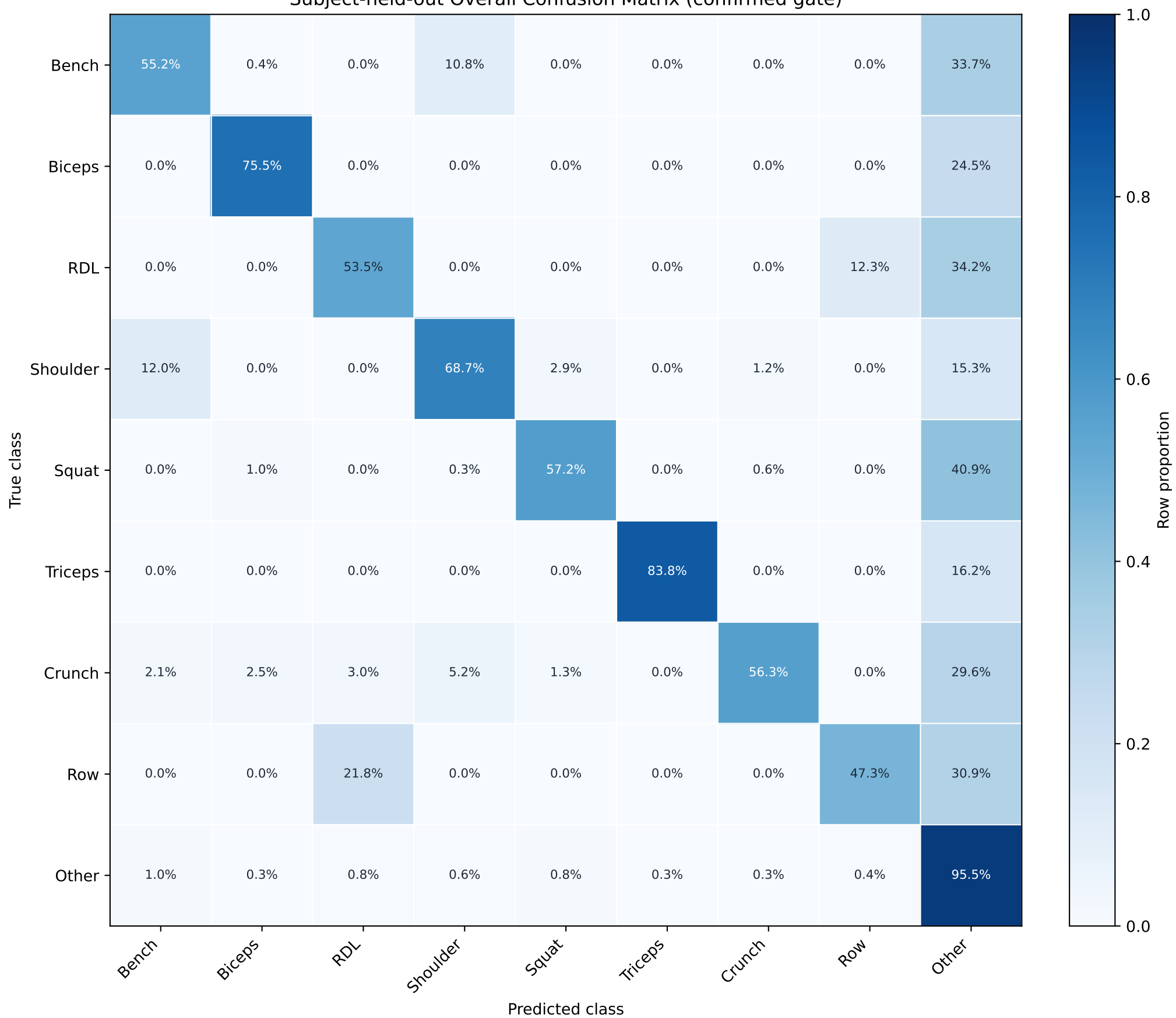
Subject-held-out Overall Confusion Matrix (confirmed gate)
