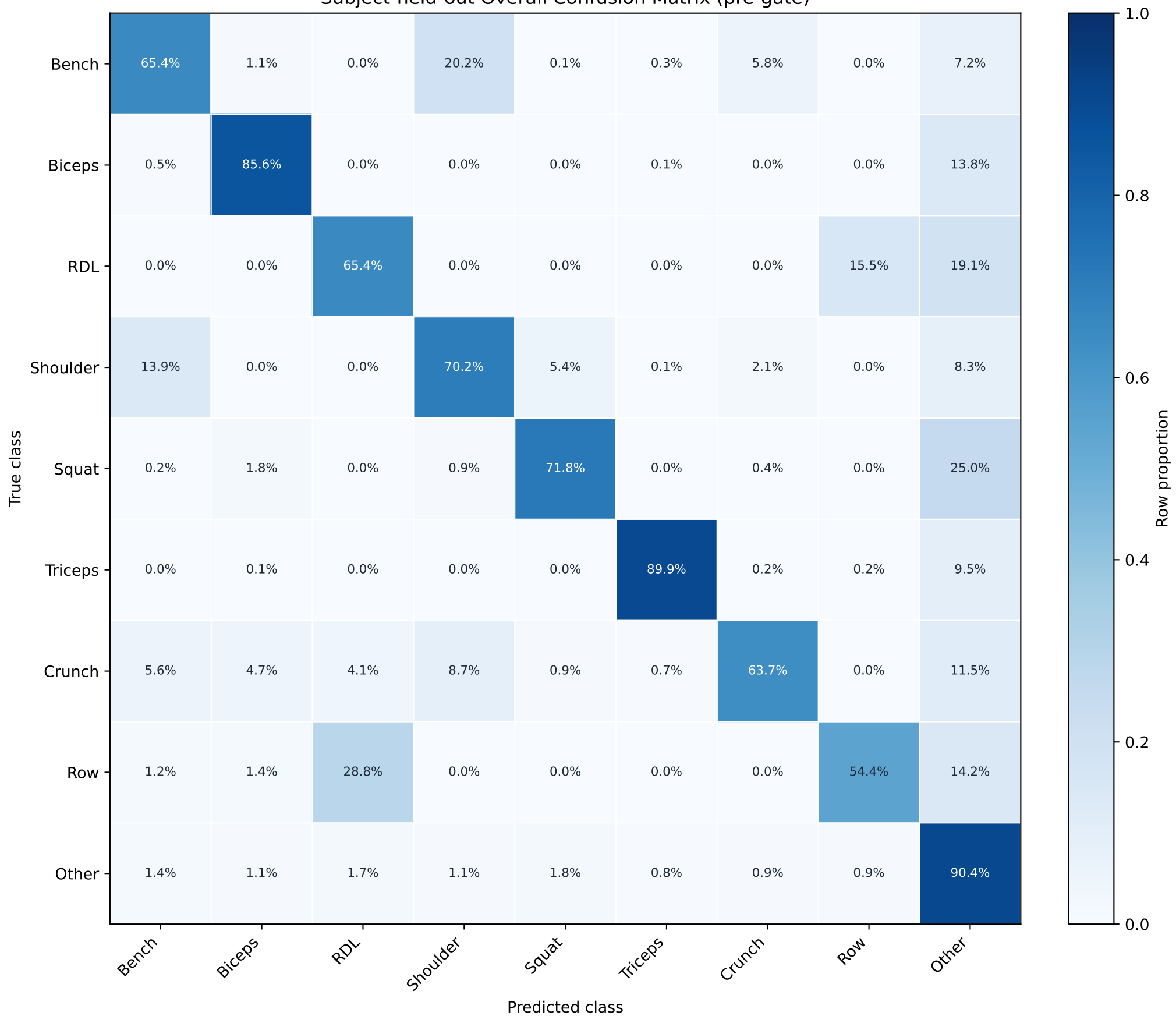
Subject-held-out Overall Confusion Matrix (pre-gate)
