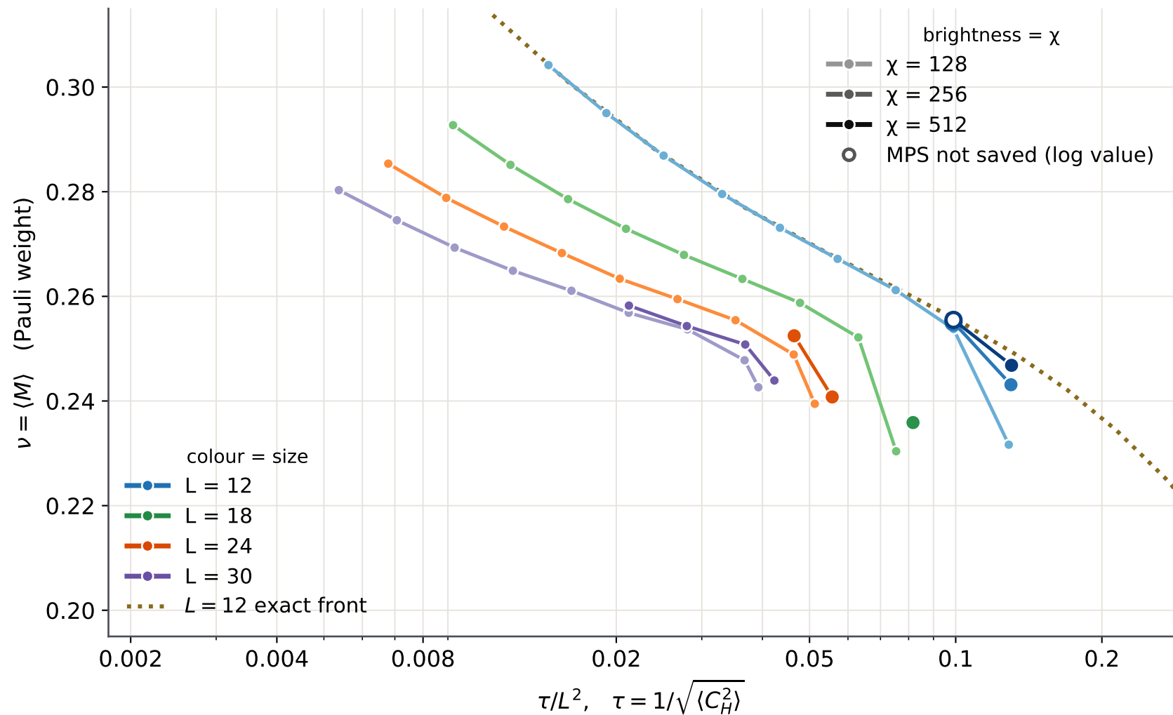
DMRG attempt: \nu vs \tau/L^2 , L = 12, 18, 24, 30 \times \chi = 128, 256, 512
