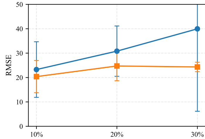
Impact of Missing Rate on Imputation Performance By Missing Pattern and Dataset
