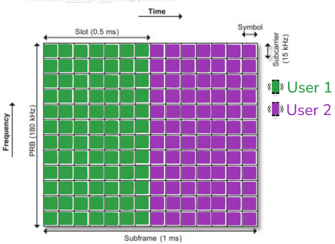
Figure 5: PRB Time and Frequency resource grid, showing how time slots are divided between users
