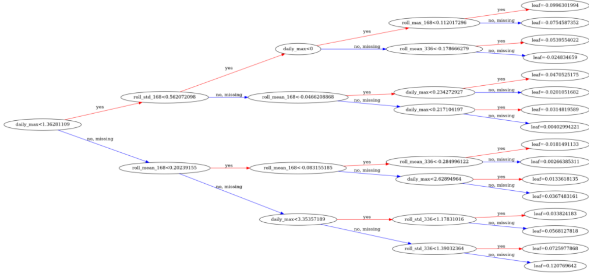
Figure 17: A single tree from XG model
