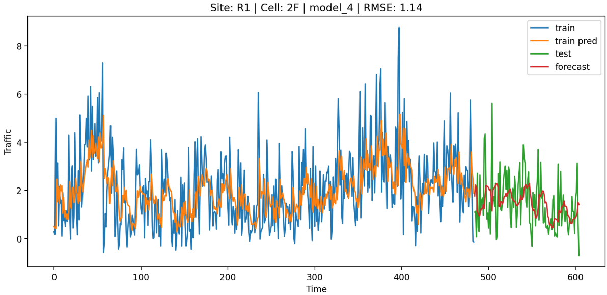
Figure 15: Seasonal Arima Fitting and Prediction on R1 2F
