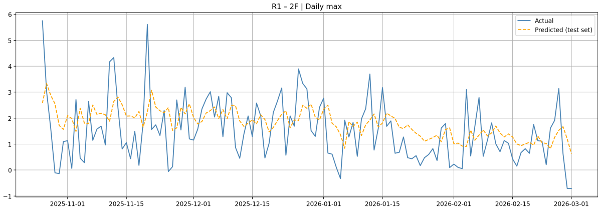
Figure 18: Prediction vs Actual, xg boost on site R1 cell 2F
