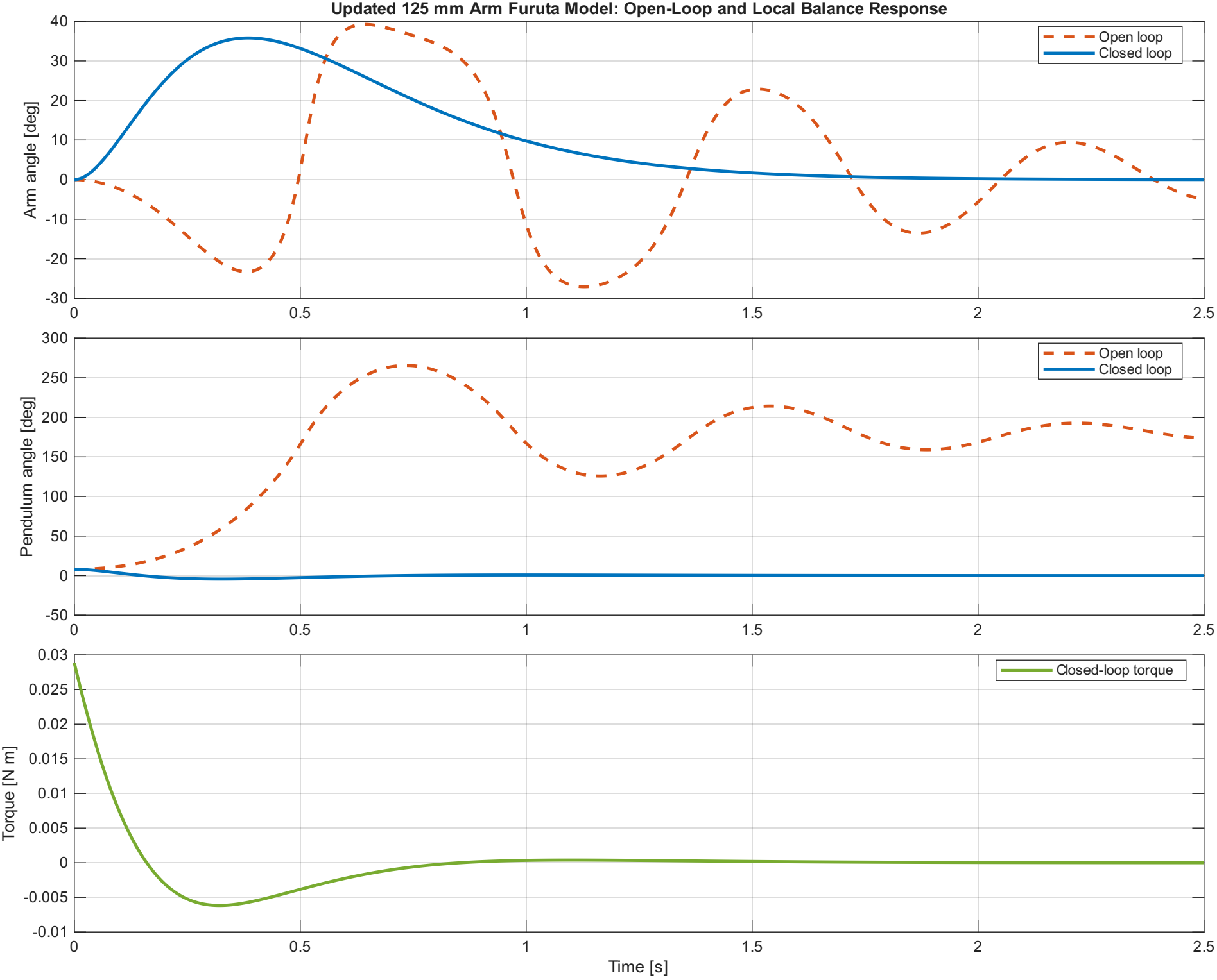
Updated 125 mm Arm Furuta Model: Open-Loop and Local Balance Response
