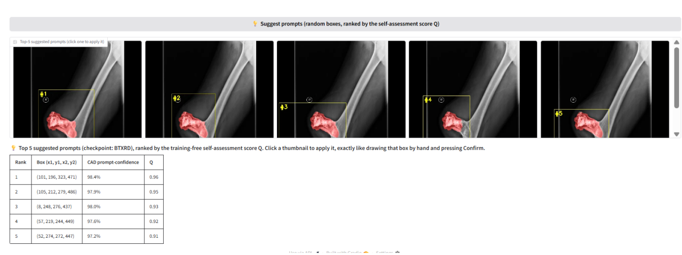
FIGURE 11. Candidate-region shortlist on a BTXRD case. Fifty boxes are sampled with no prompt, scored by the self-assessment score Q , and the five highest-scoring boxes are shown for the clinician to accept, adjust, or reject. A FracAtlas case is shown in the supplementary material.
