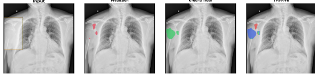
FIGURE 10. Failure case on BTXRD (IMG000013, Dice 0.120): the prompt covers the lesion at the chest/rib margin, but PGA-UNet's prediction lands away from it. A covering box does not fix a case where the local image evidence is itself ambiguous.
