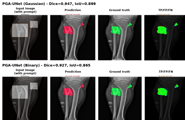
FIGURE 5. Representative qualitative comparison between the Gaussian prompt representation and the binary prompt representation. The figure illustrates a case in which the Gaussian version yields cleaner boundaries and better overlap.
