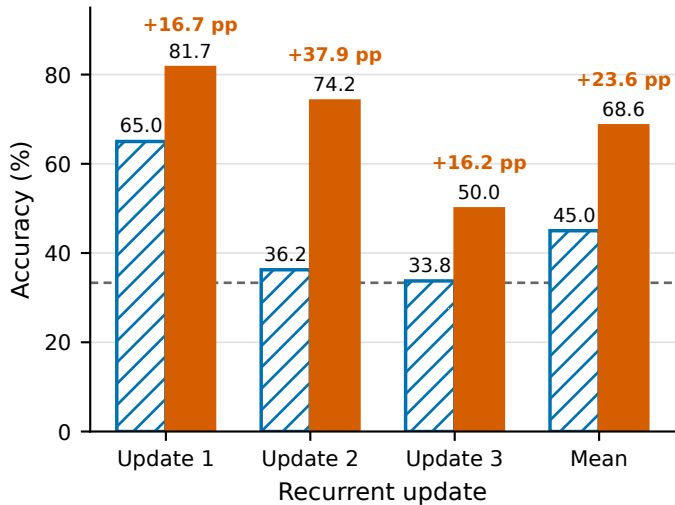
(b) Final stage-wise accuracy
