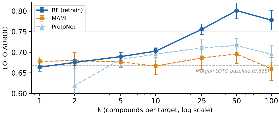
(a) Macro-mean across evaluable targets (cohort 65→14, 10 seeds; \pm 1 SD)
