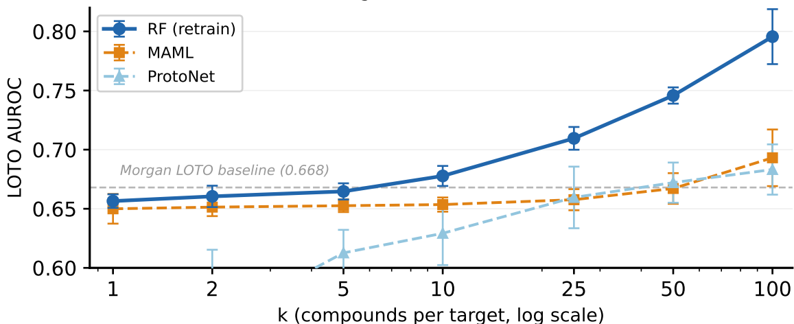
(b) Matched cohort (n=14 targets, 10 seeds; \pm 1 SD)
