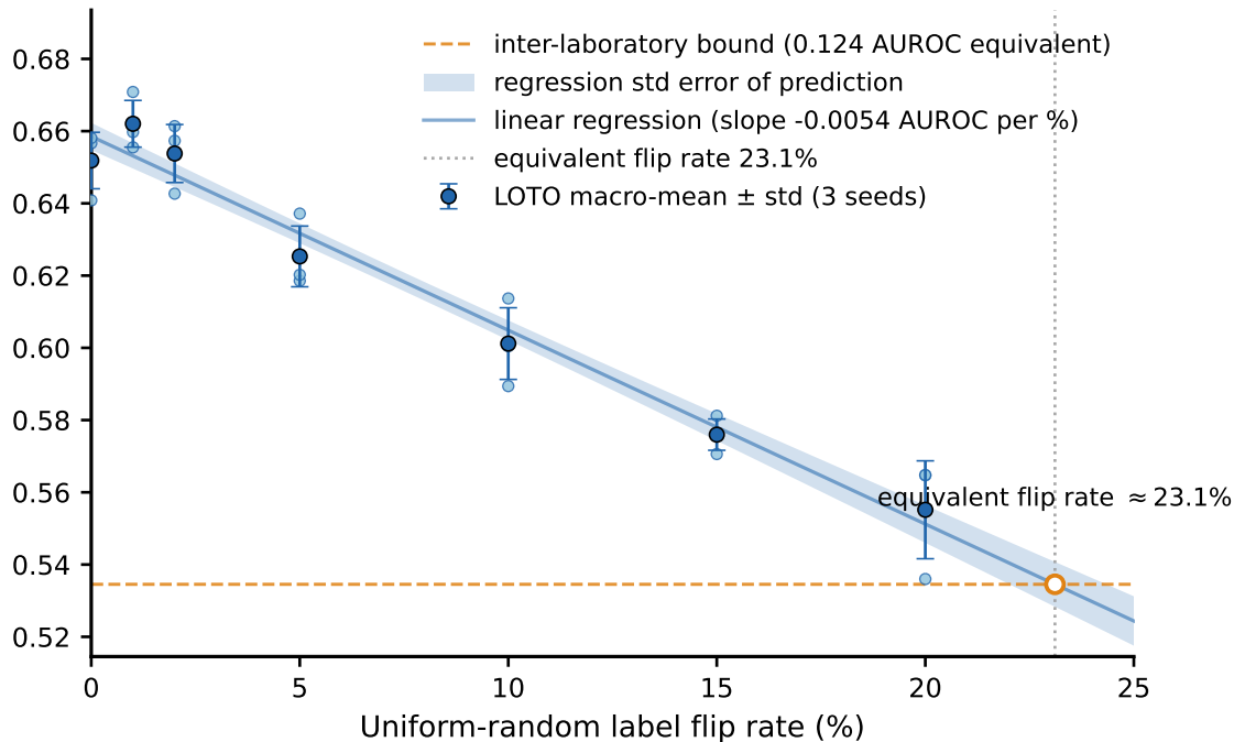
LOTO macro-mean AUROC
