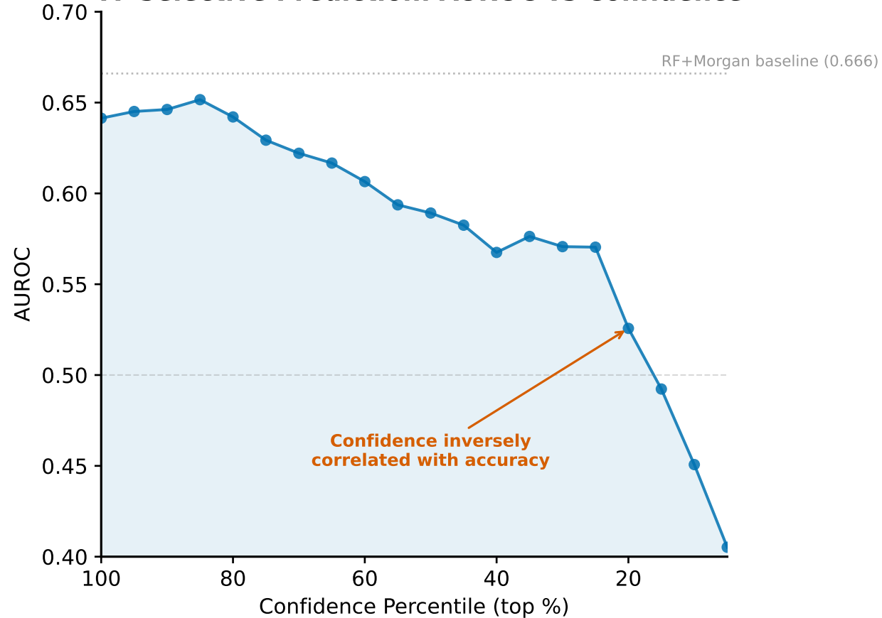
A Selective Prediction: AUROC vs Confidence
