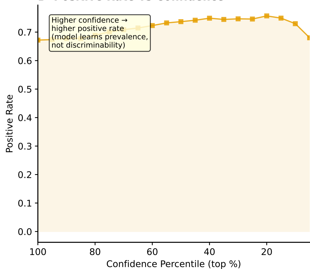
B Positive Rate vs Confidence
