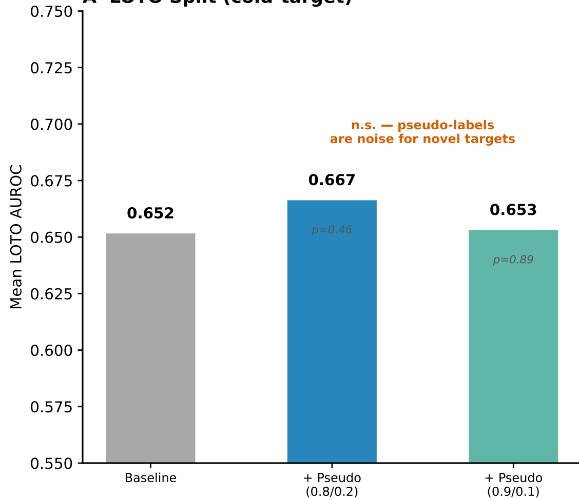
A LOTO Split (cold-target)
