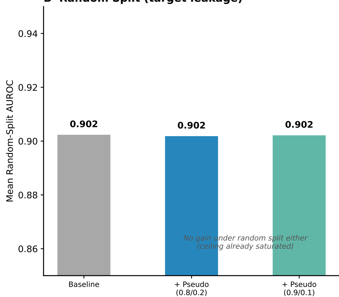
B Random Split (target leakage)
