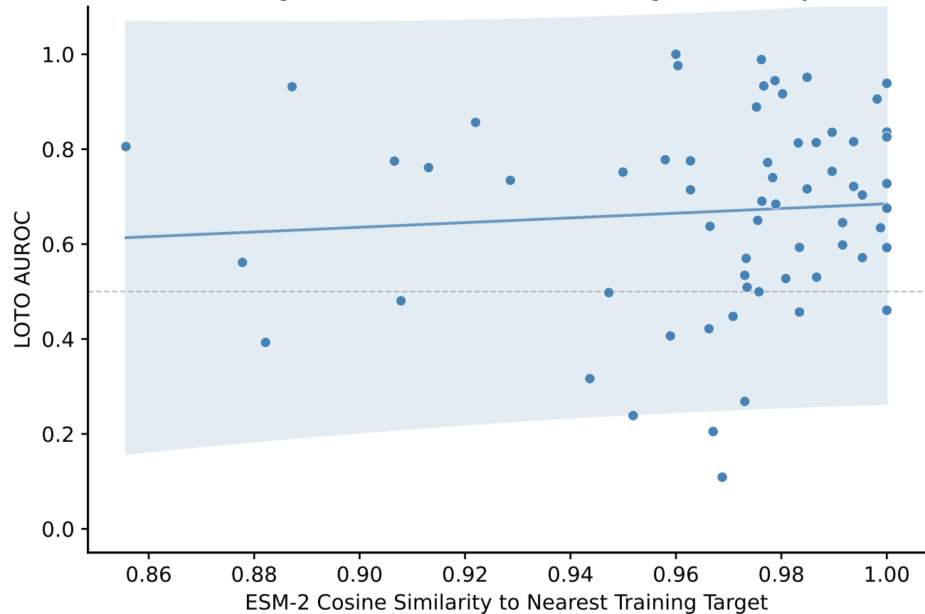
Per-Target LOTO Performance vs. Target Similarity
