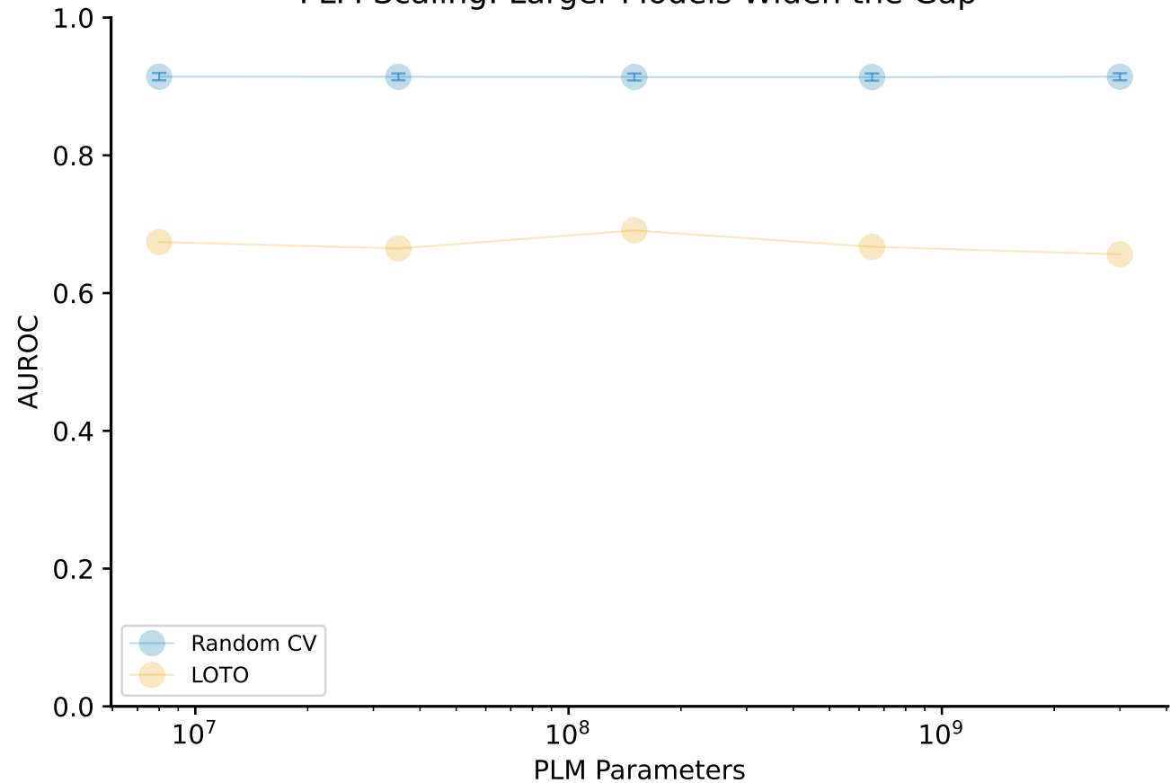
PLM Scaling: Larger Models Widen the Gap
