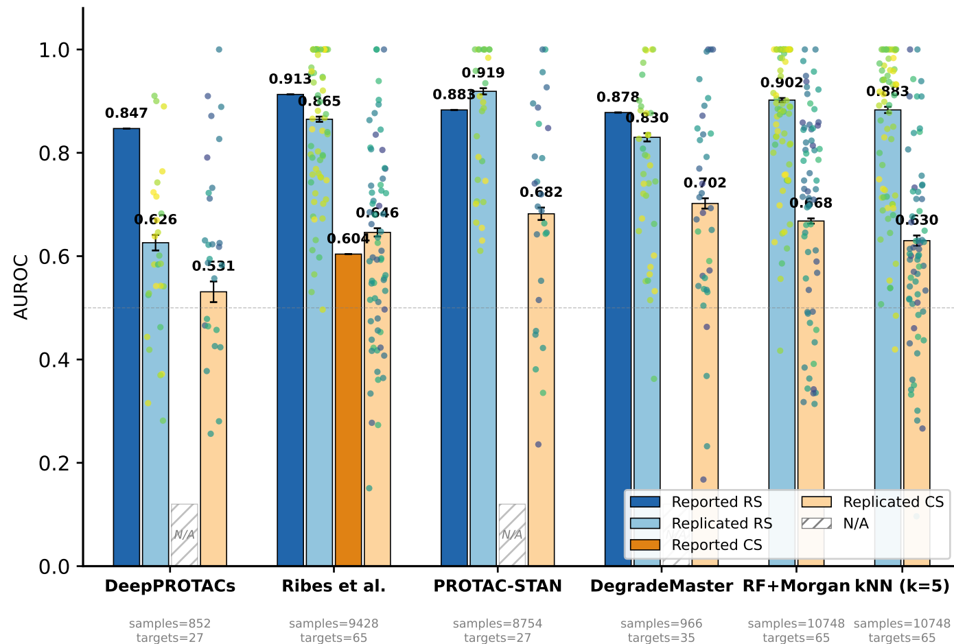
A Reported vs. Replicated Performance
