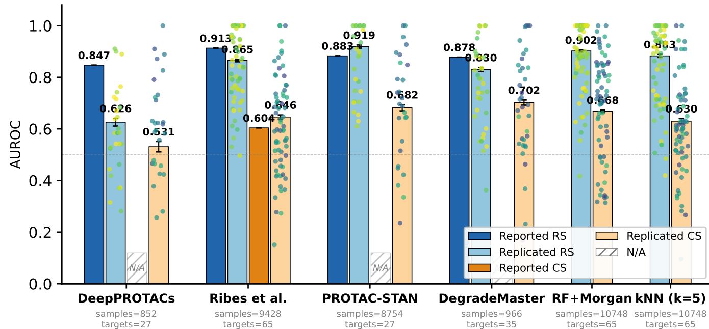
A Reported vs. Replicated Performance
