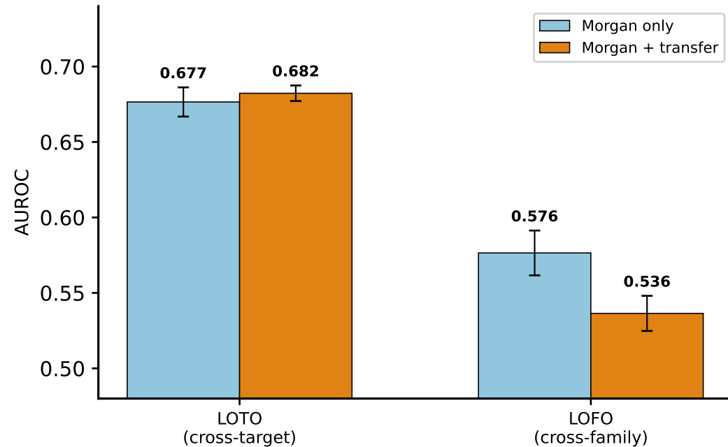
B LOTO vs LOFO
