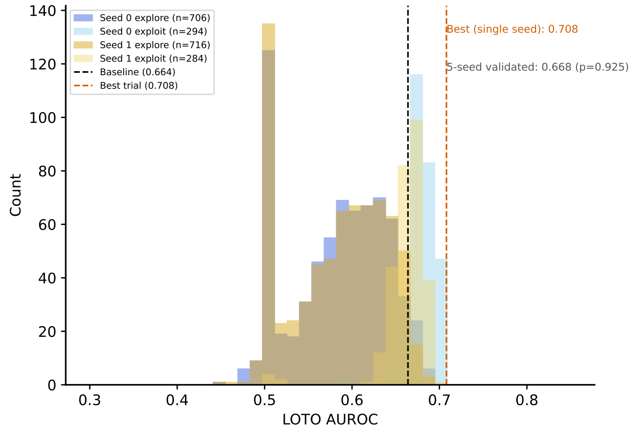
A HPO Trial Distribution
