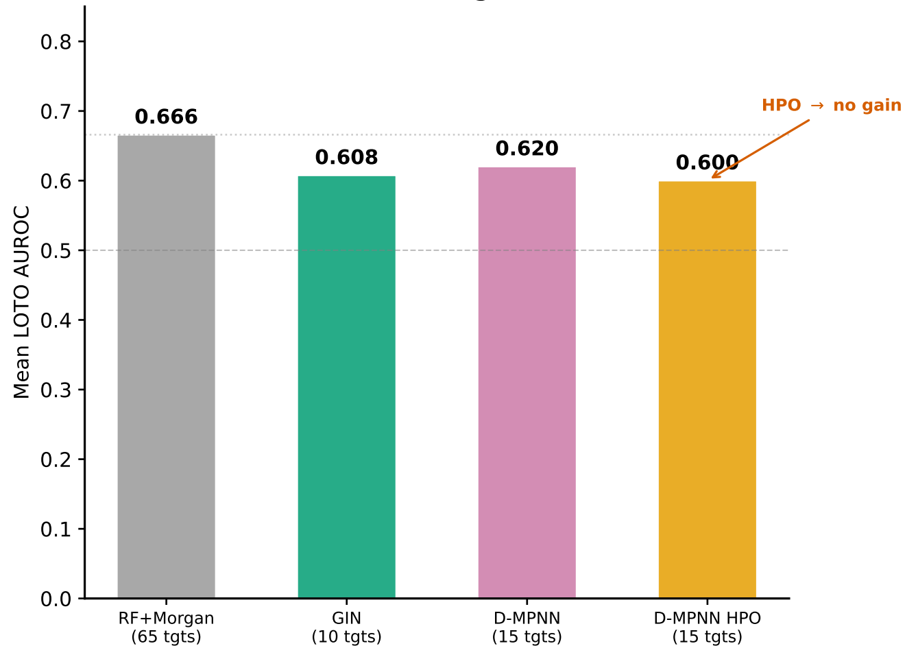
A GNN Baselines vs RF+Morgan
