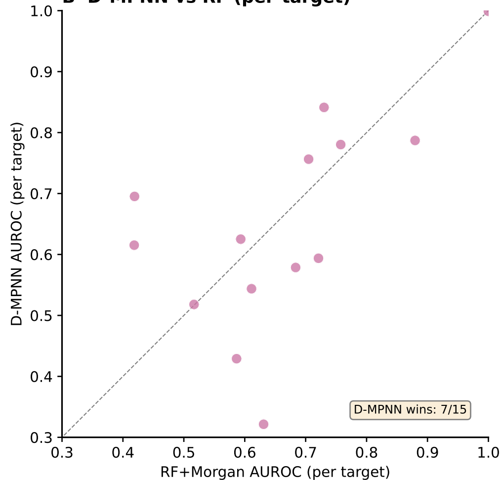
B D-MPNN vs RF (per-target)
