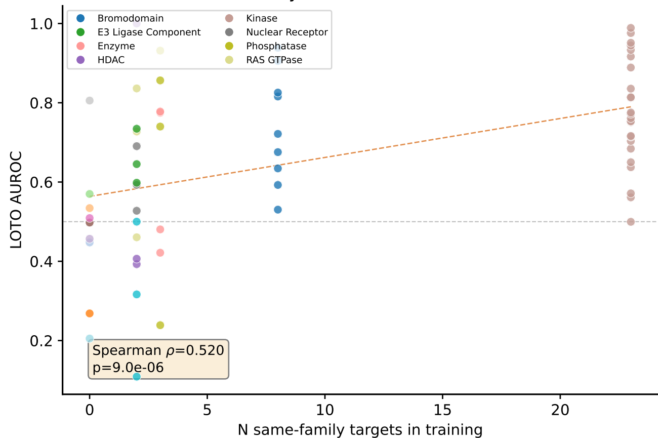
Protein Family Size vs. LOTO Performance
