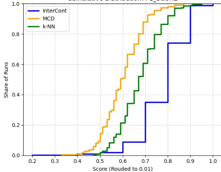
Cumulative Distribution: F1_SCORE
