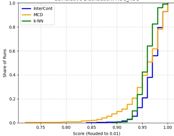
Cumulative Distribution: ROC_AUC
