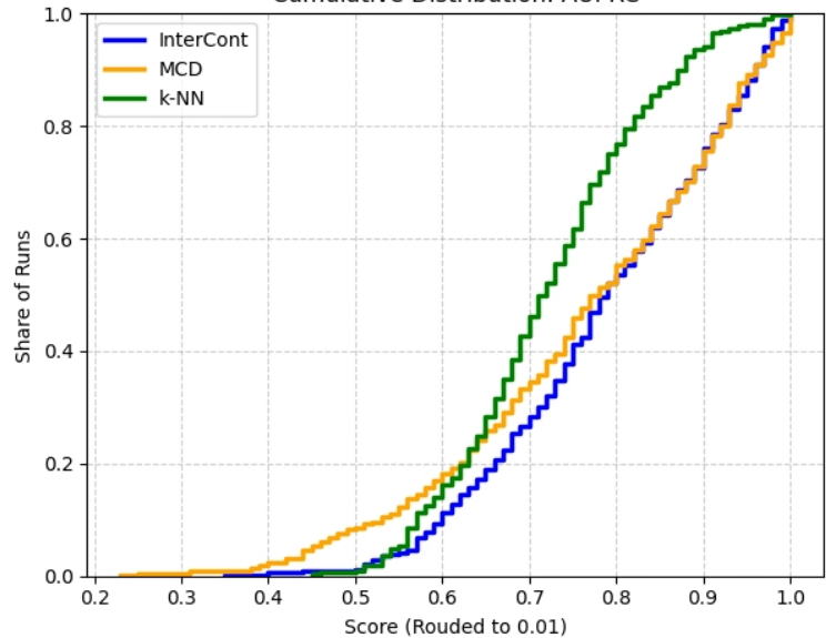
Cumulative Distribution: AUPRC
