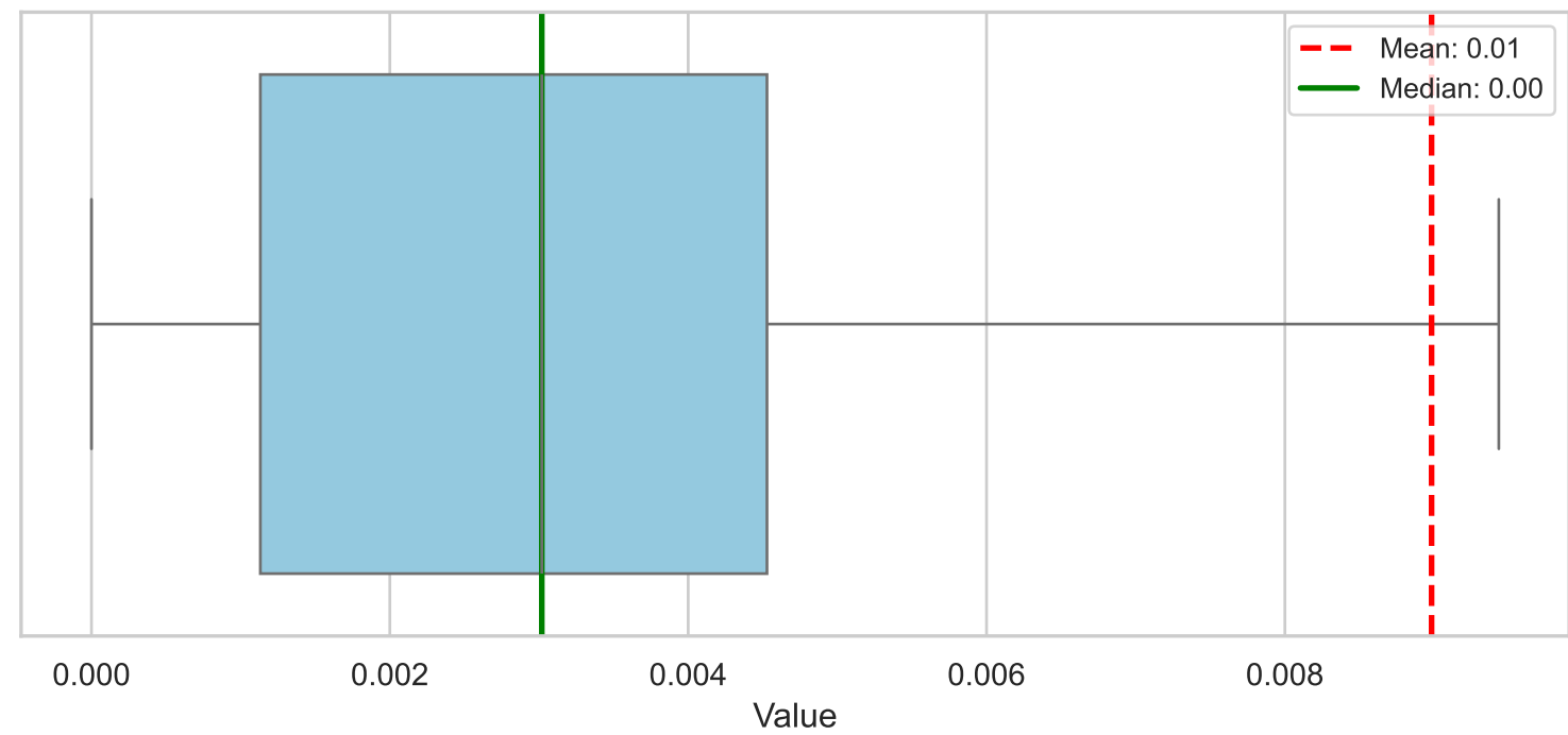
Feature 3
