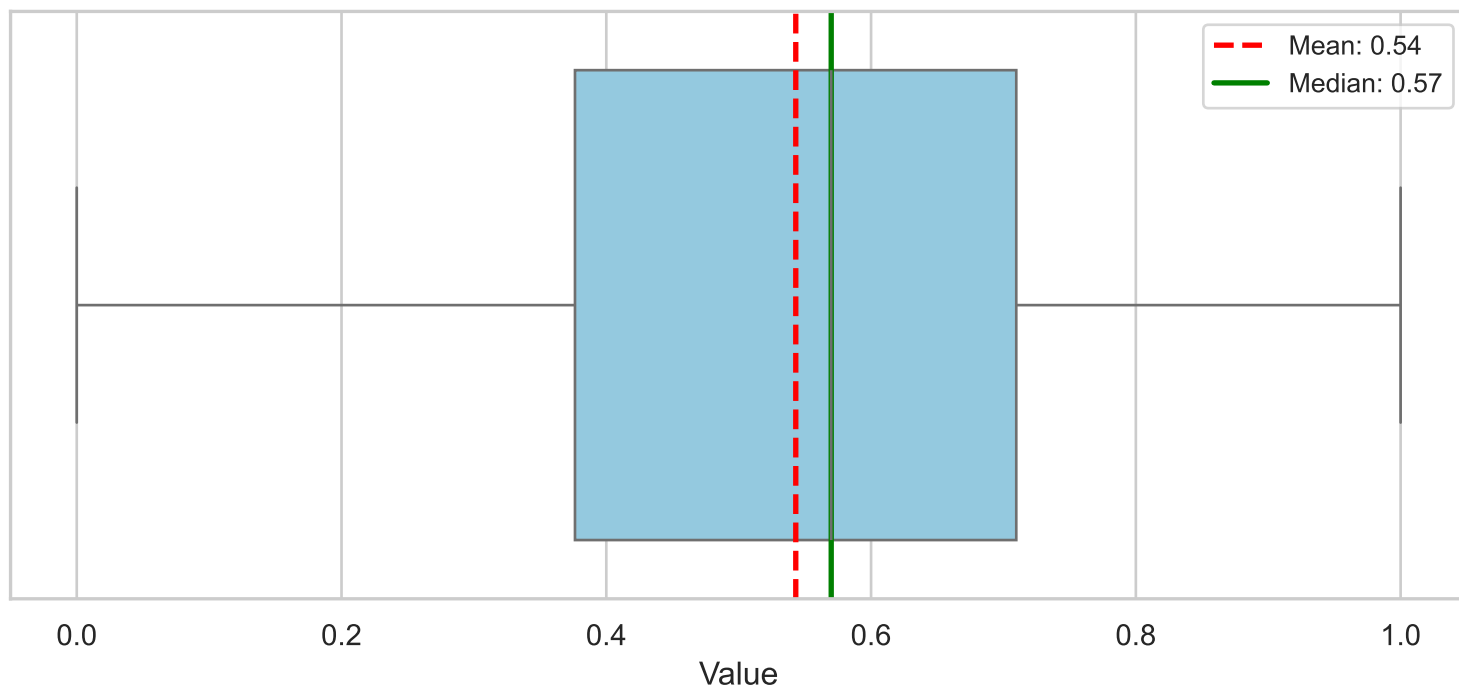
Feature 2
