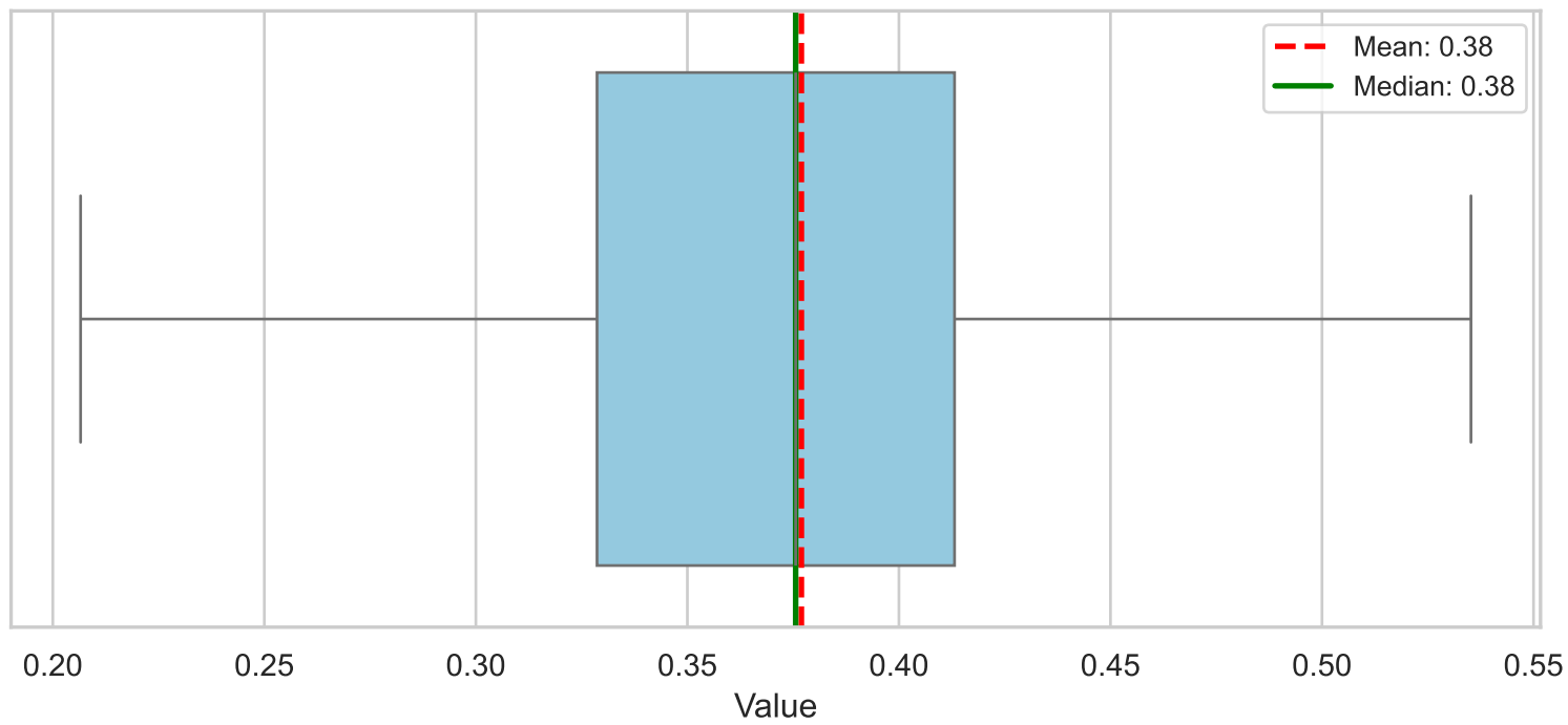
Feature 4
