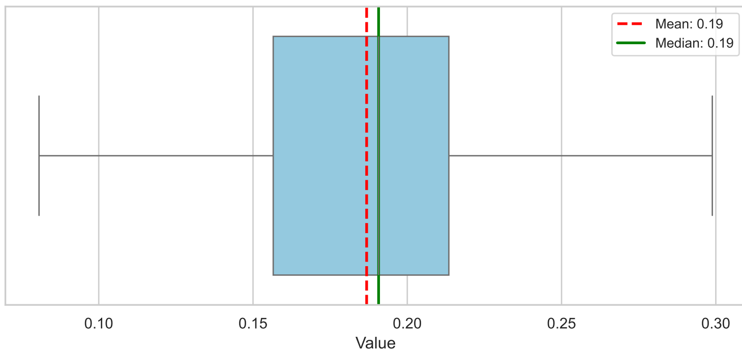
Feature 4
