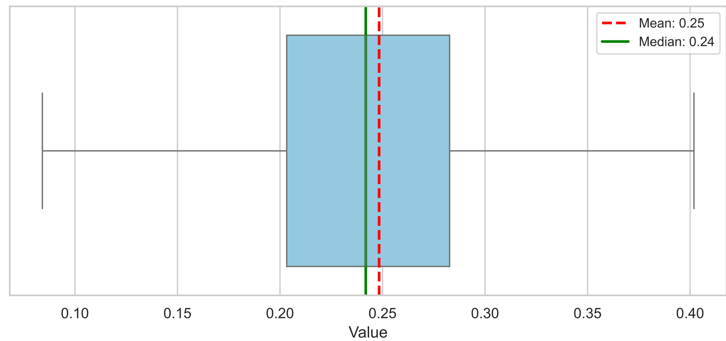
Feature 5
