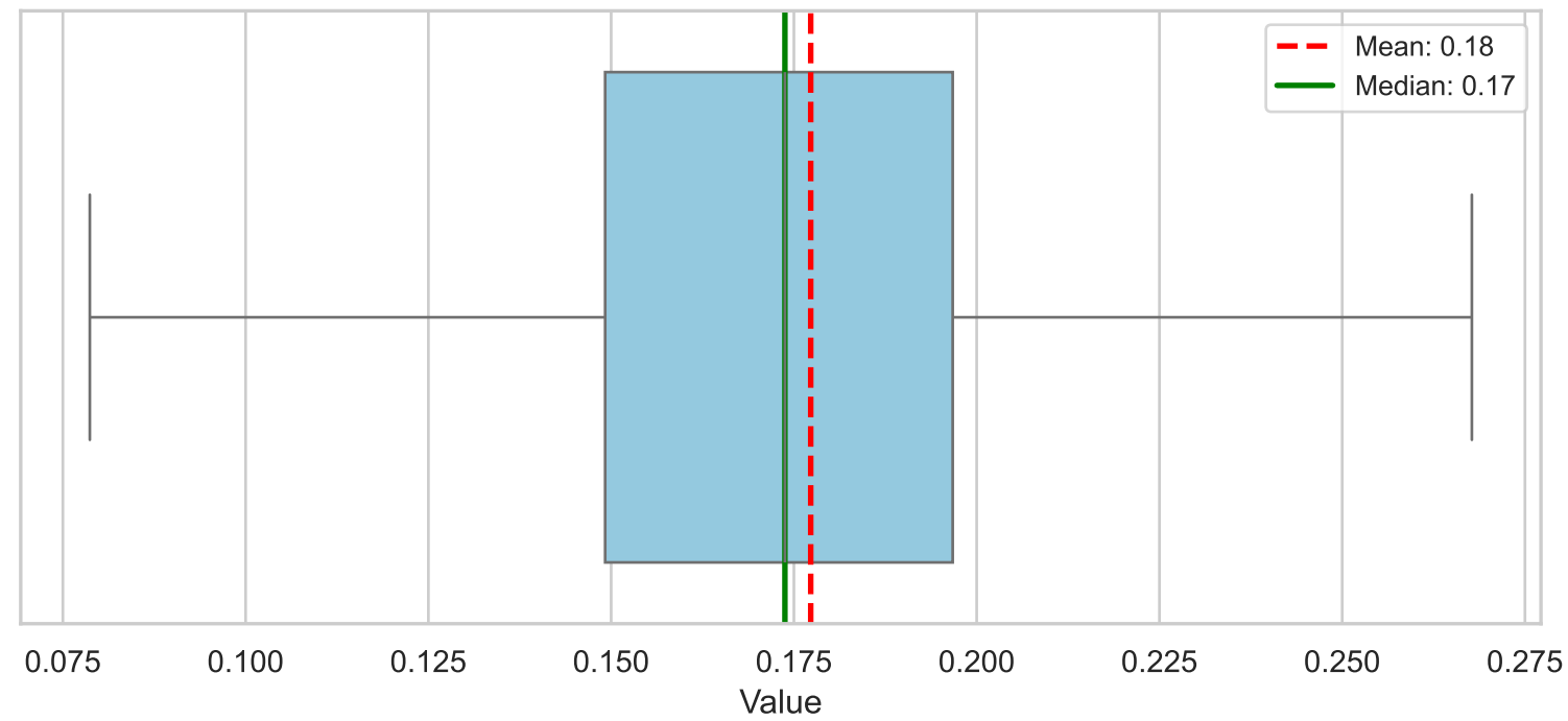
Feature 5
