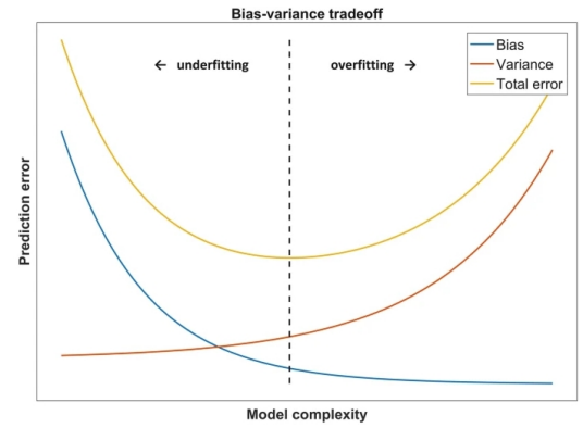
Figure 3: Bias-Variance Tradeoff.
