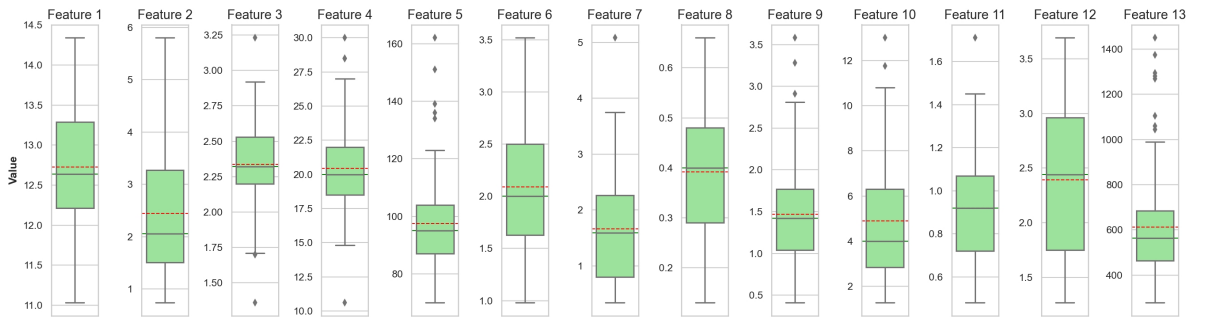
Figure 10: Boxplots per Dimension
