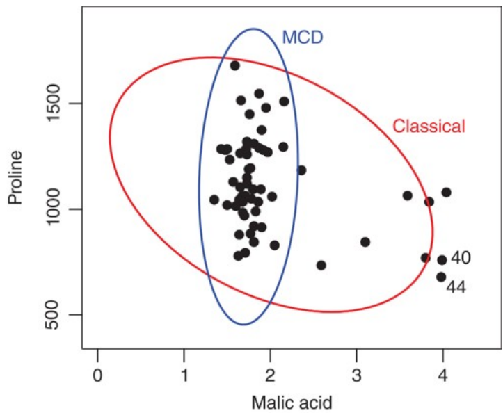
Figure 8: Minimum Covariance Determinant.
