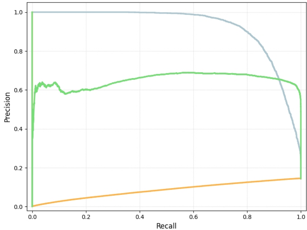
Precision-Recall
