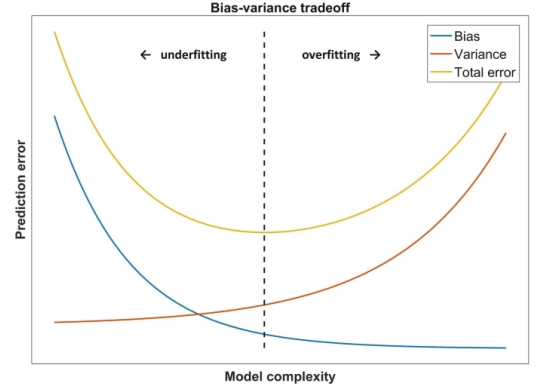
Figure 3: Bias-Variance Tradeoff.
