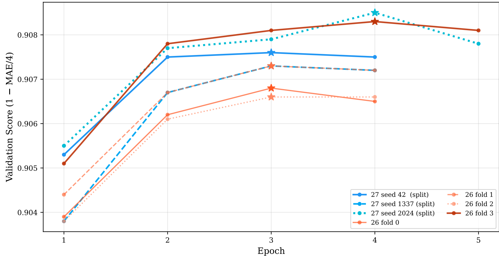
Learning Curves — Baselines 26 (k-fold) and 27 (seed-split)
