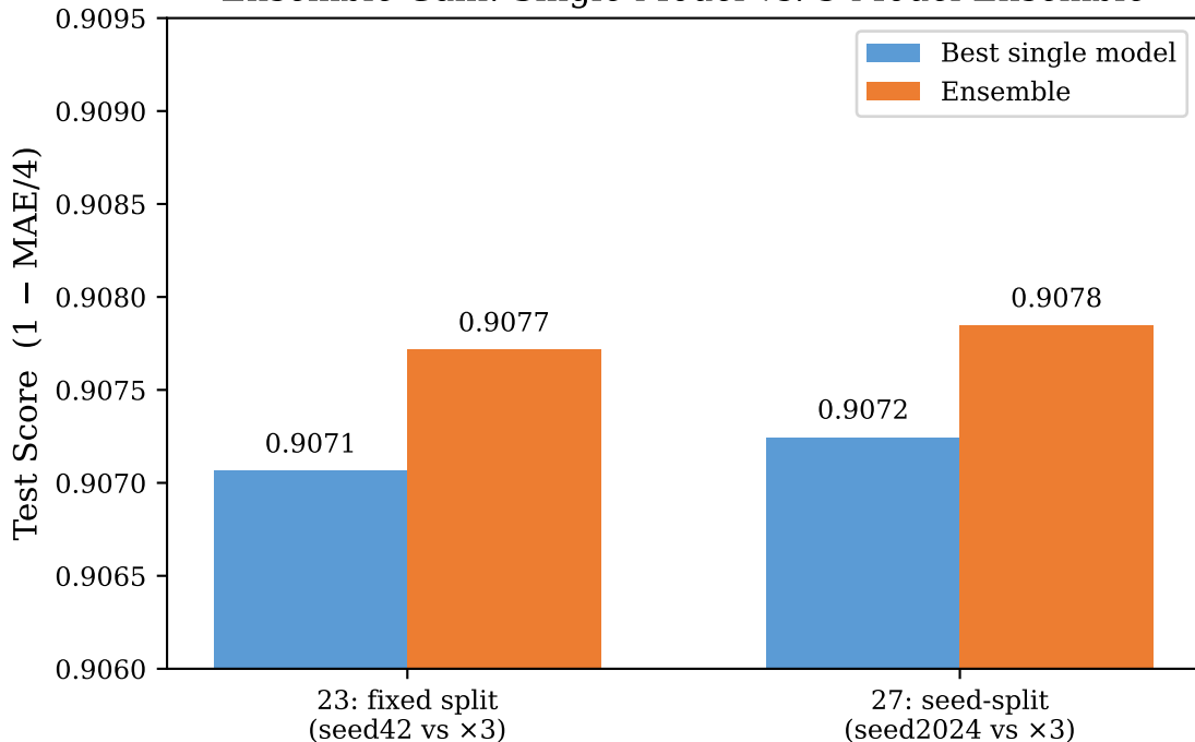
Ensemble Gain: Single Model vs. 3-Model Ensemble
