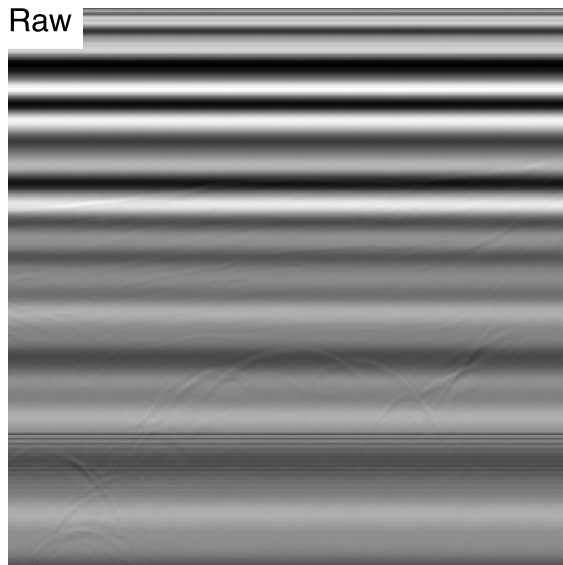
Mean subtracted
