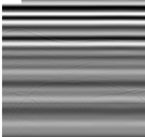
Mean subtracted
