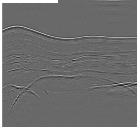
RPCA, \lambda = 1.00
