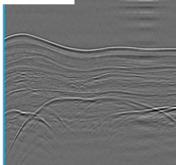
RPCA, \lambda = 0.25
