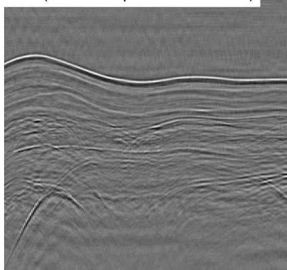
SVD (first 5 components removed)
