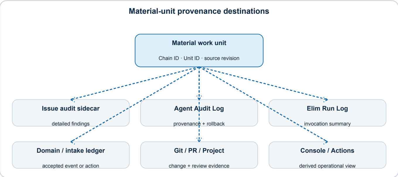
Figure: Material-unit provenance destinations. Arrows show data or control flow, not grants of authority.
