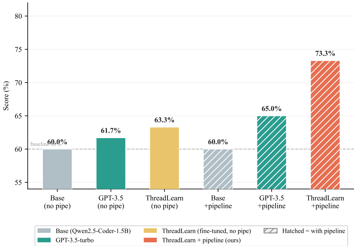
Ablation: Score by Configuration on 30-Case Real-World Benchmark
