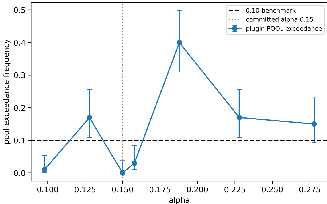
F11 plugin pool alpha sweep -- mnist ts0 greedy
