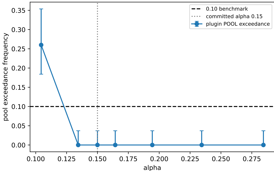
F11 plugin pool alpha sweep -- tabular-MiniBooNE ts0 greedy
