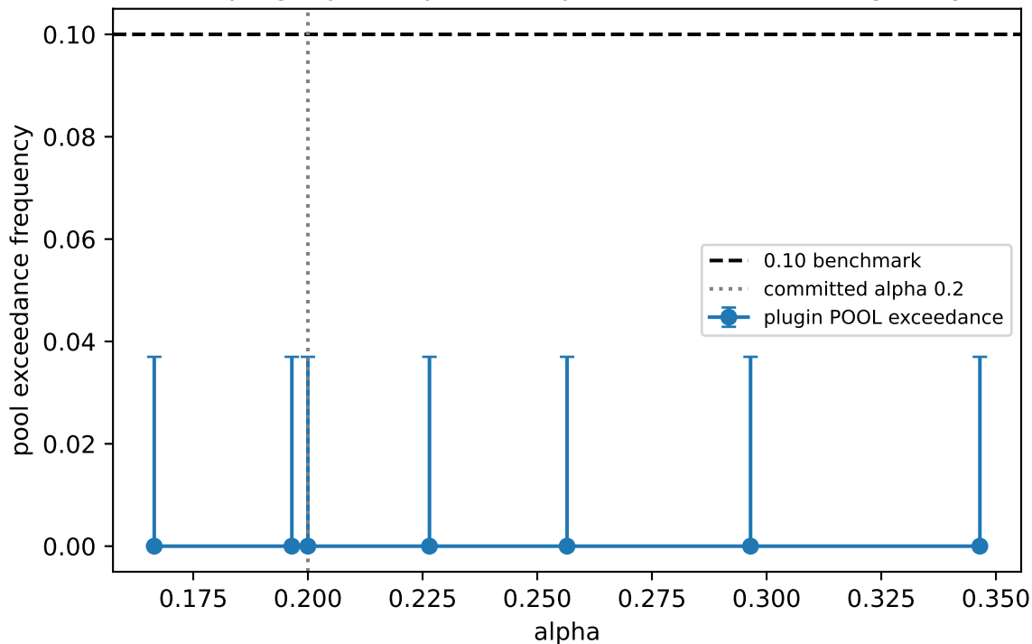
F11 plugin pool alpha sweep -- tabular-adult ts0 greedy
