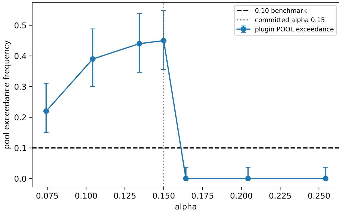
F11 plugin pool alpha sweep -- tabular-spambase ts0 greedy
