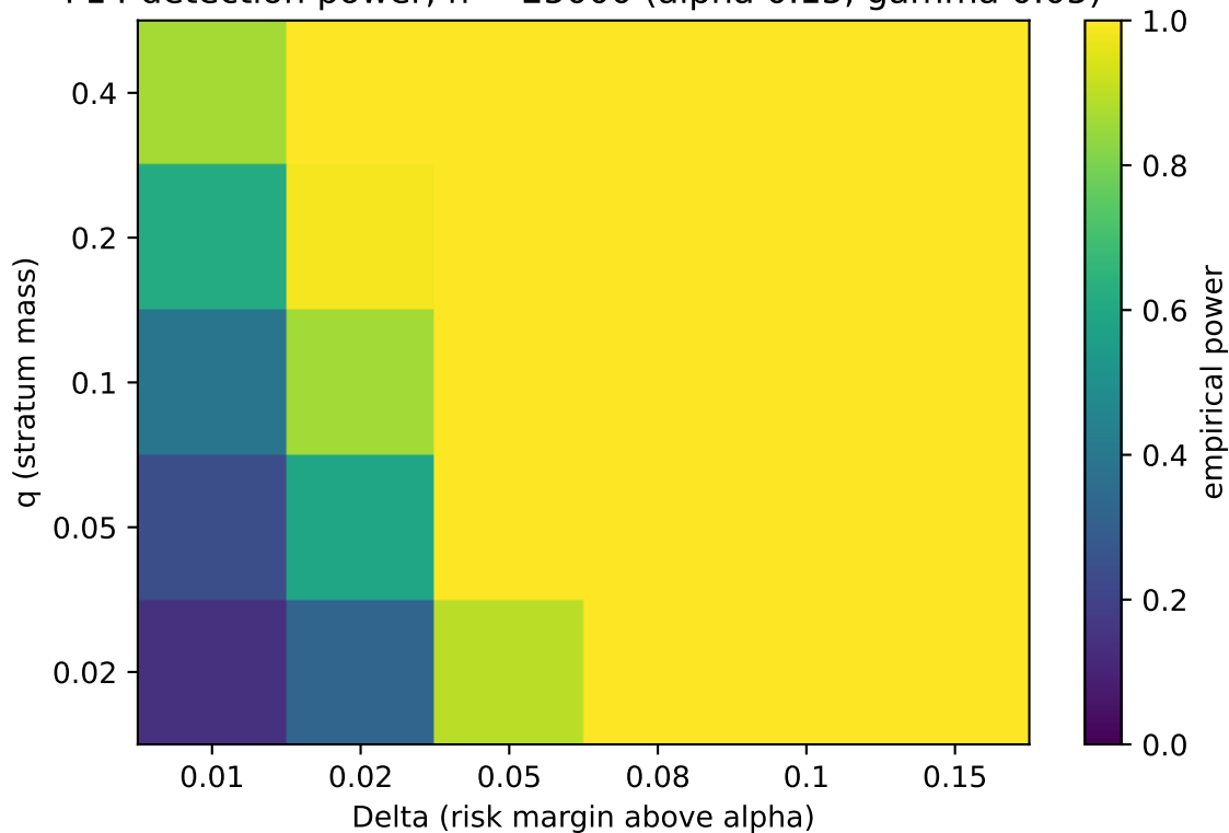
F14 detection power, n = 25000 (alpha 0.15, gamma 0.05)
