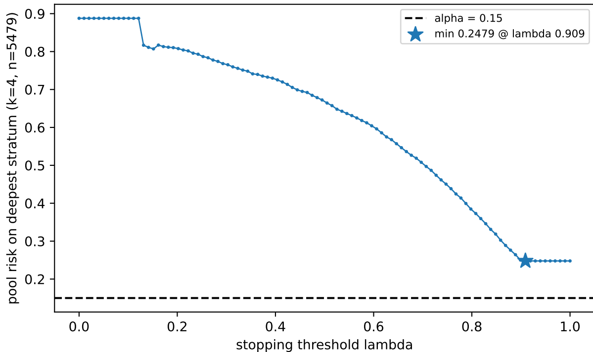
F8 threshold-family risk -- mnist ts0 greedy, lr=0.9
