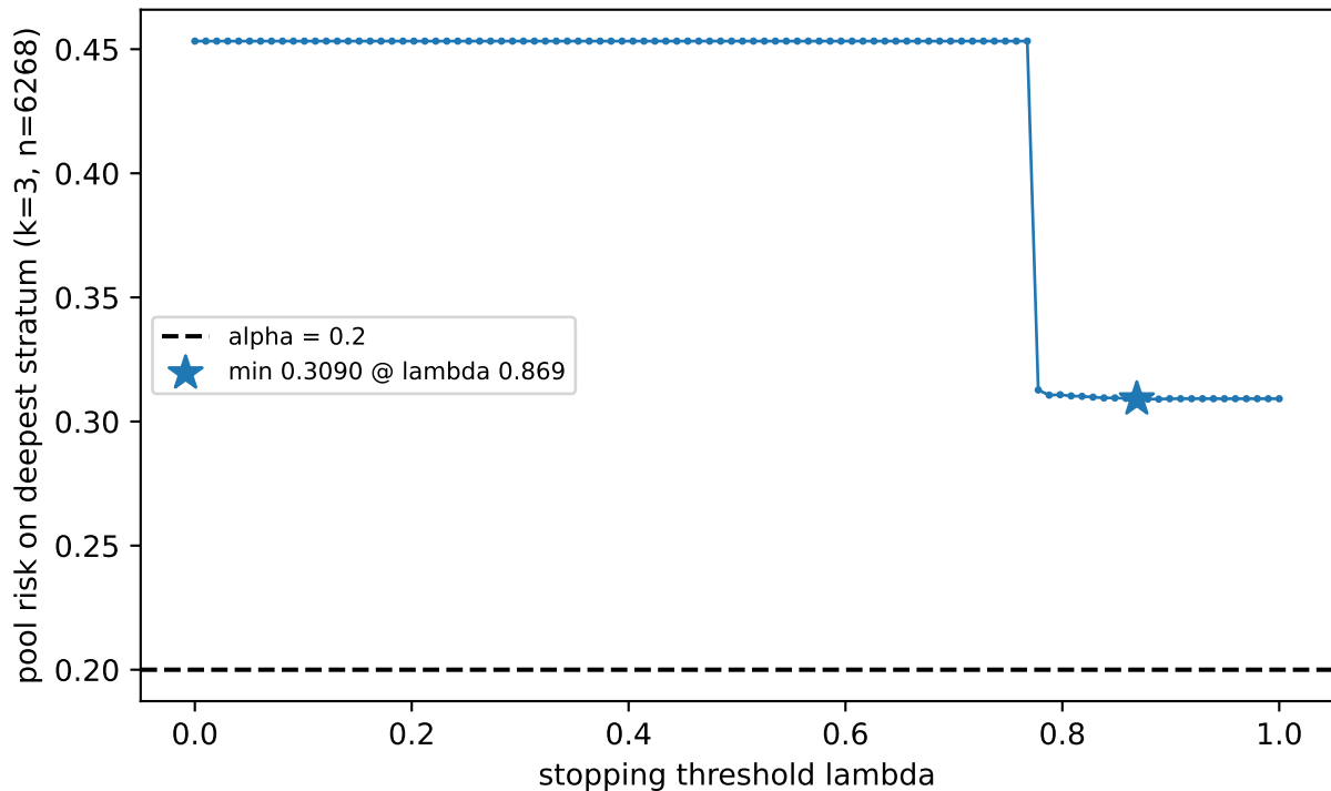
F8 threshold-family risk -- tabular-adult ts0 greedy, lr=0.9
