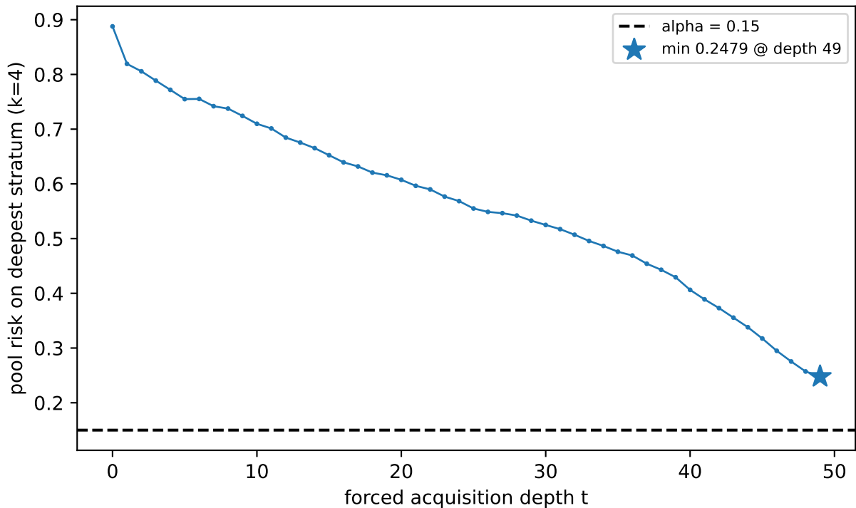
F9 forced-depth risk -- mnist ts0 greedy, lr=0.9
