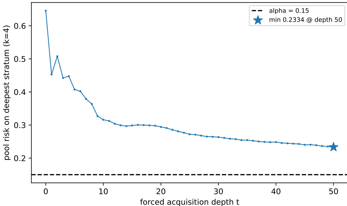
F9 forced-depth risk -- tabular-MiniBooNE ts0 greedy, lr=0.9
