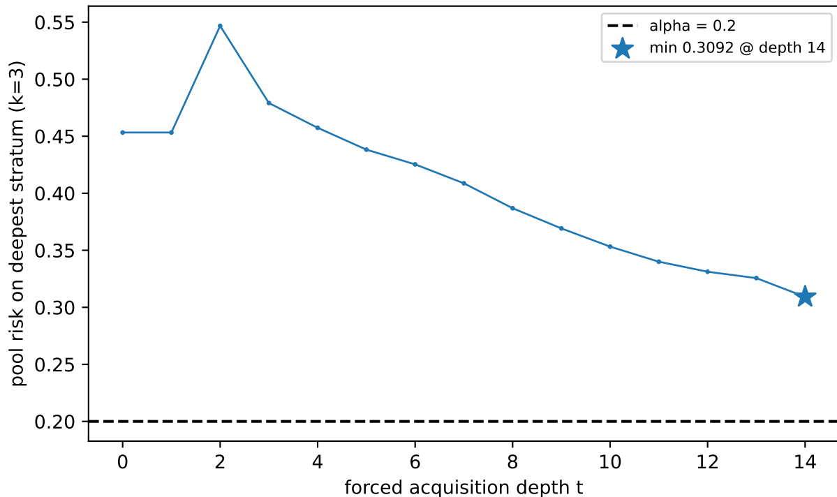
F9 forced-depth risk -- tabular-adult ts0 greedy, lr=0.9
