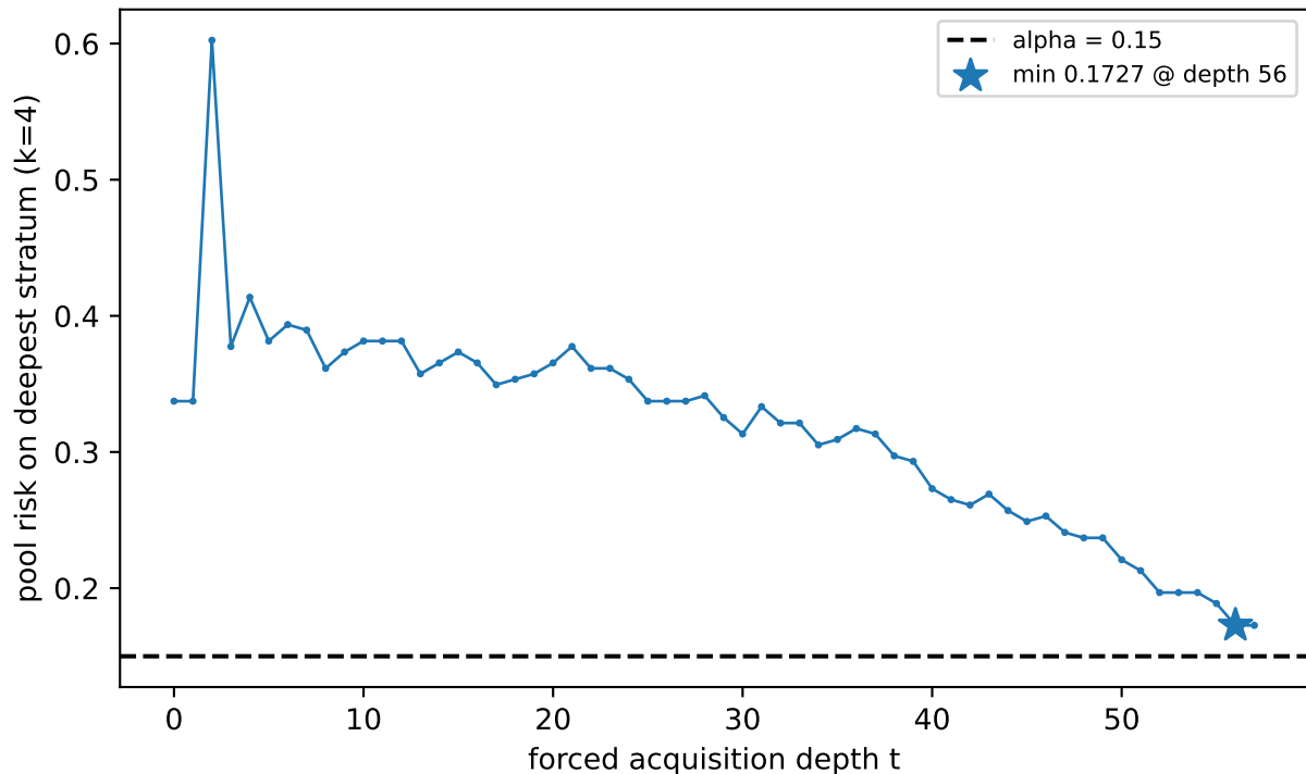
F9 forced-depth risk -- tabular-spambase ts0 greedy, lr=0.9
