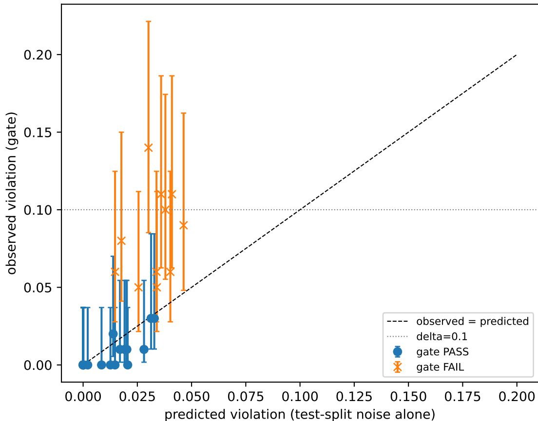
F6 validity diagnostic -- predicted vs observed marginal violations
