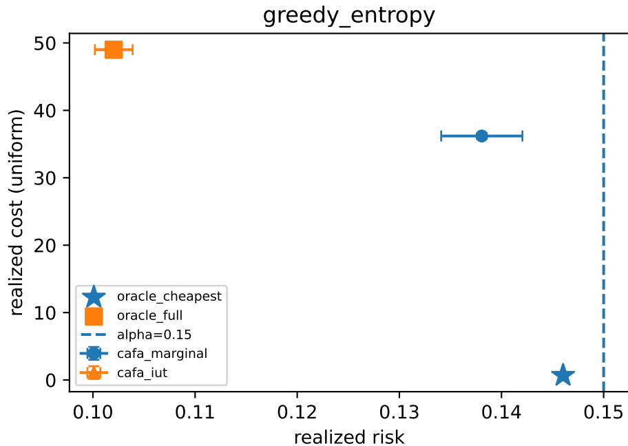
F1 realized (risk, cost) -- mnist ts2 (lambda_ref=0.9)
