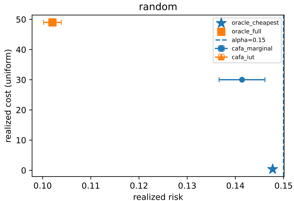
F1 realized (risk, cost) -- mnist ts2 (lambda_ref=0.9)
